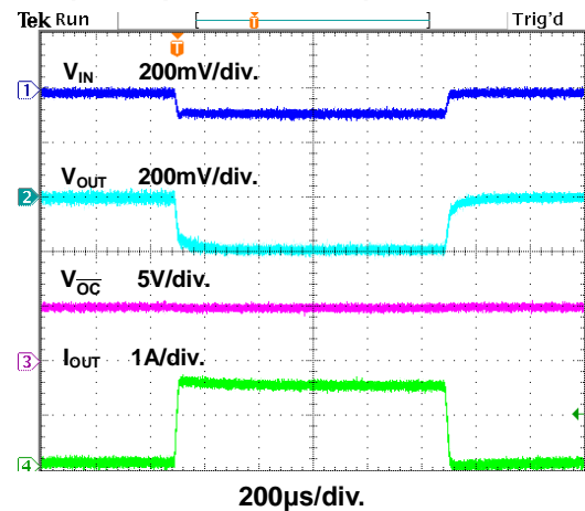
Figure 12. Load transient
