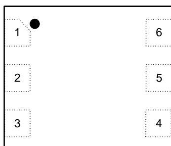
Figure 2 Top view
