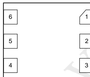
Figure 3 Bottom view
