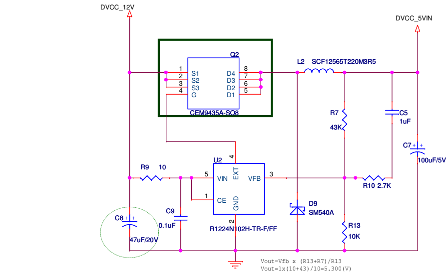
12V to 5V/3A DCDC circuit diagram
