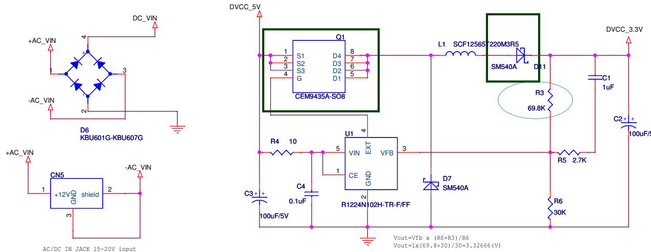
5V to 3.3V/3A DCDC circuit diagram
