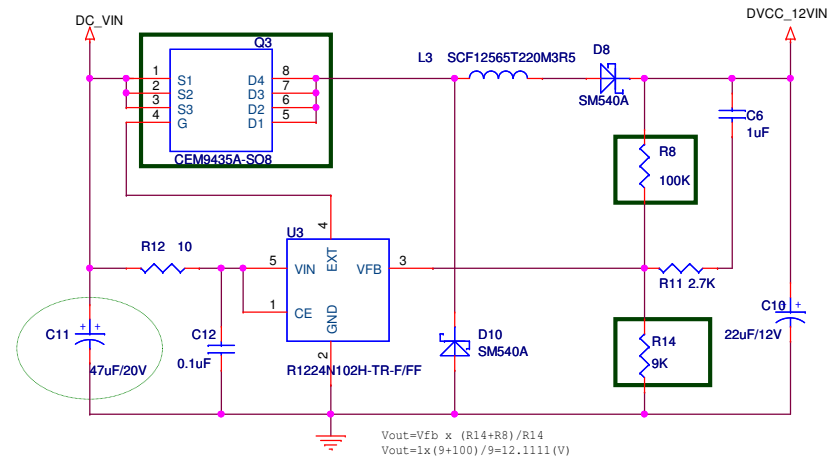
12V~20V to 12V/3A DCDC circuit diagram
