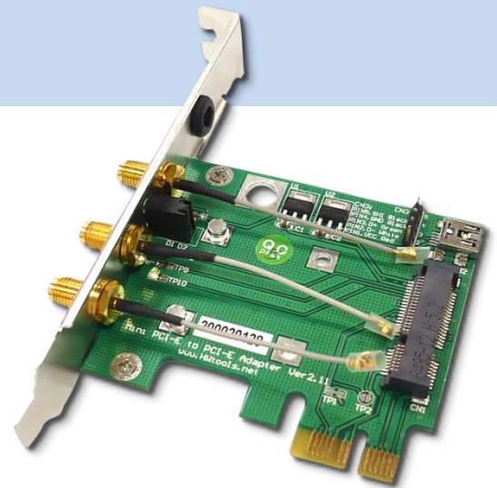
u.FL/IPX (Mini-PCI) to RP-SMA pigtail WiFi RF cable adapter
