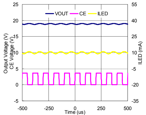
R1205N823B(CE Freq=10KHz)
