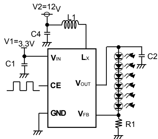
Fig 2. R1205x8xxB
