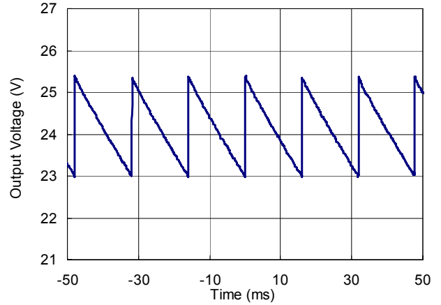
R1205N823B(CE Freq=10KHz)
