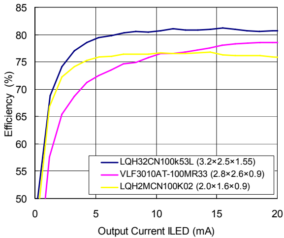
6LED, V IN =3.6V
