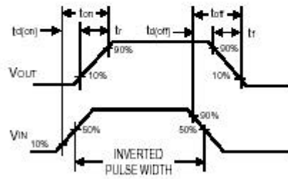
Figure 12. Switching Waveforms
