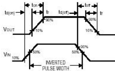
Figure 12. Switching Waveforms
