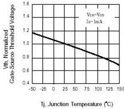
Figure 5. Gate Threshold Voltage with Temperature
