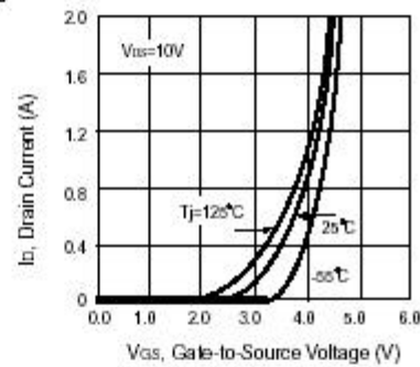
Figure 2. Transfer Characteristics
