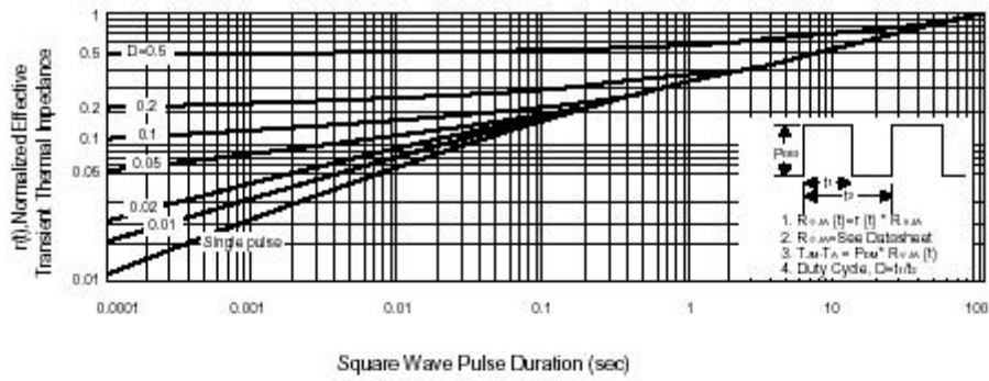
Figure 13. Normalized Thermal Transient Impedance Curve
