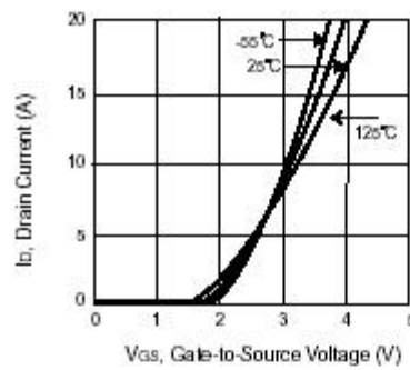
Figure 2. Transfer Characteristics
