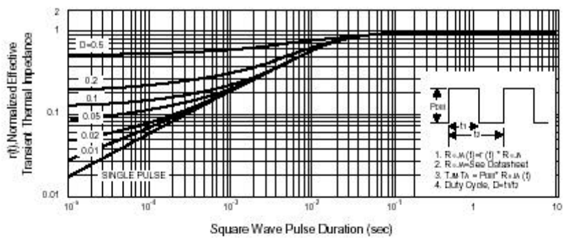
Figure 13. Normalized Thermal Transient Impedance Curve
