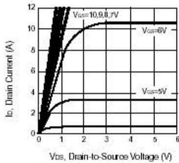
Figure 1. Output Characteristics
