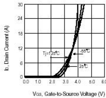
Figure 2. Transfer Characteristics
